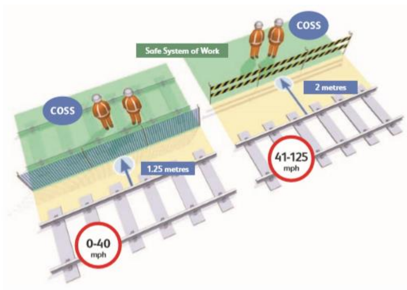
Examples of fenced Safe System of Work – (left) using plastic netting on a blocked line and (right) using barricade tape in the cess.
